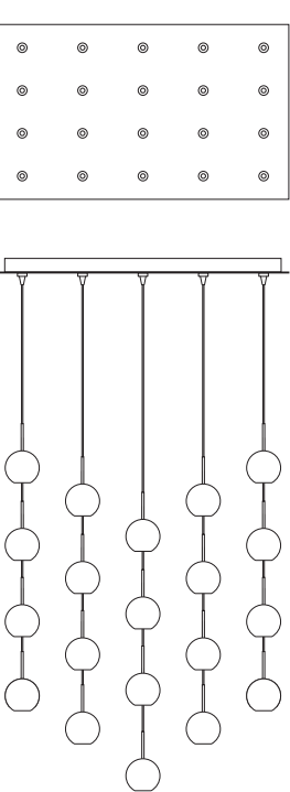
CPEJRT20(FINISH)1831(HAL, LED) EZ JACK FINISH LAMP DIMENSIONS
