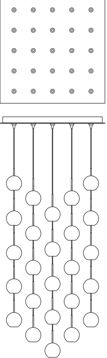
CPEJSQ25(FINISH)(HAL, LED) EZ JACK FINISH LAMP DIMENSIONS
