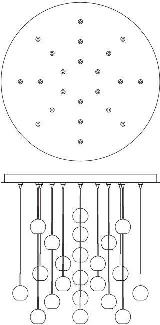
CPEJRN21(FINISH)26(HAL, LED) EZ JACK FINISH LAMP DIMENSIONS
