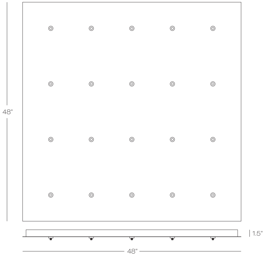
CPEJSQ20(F)4848(L) 20 Lights
